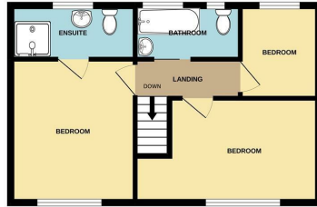
1ST FLOOR 406 sq.ft. (37.7 sq.m.) approx.
